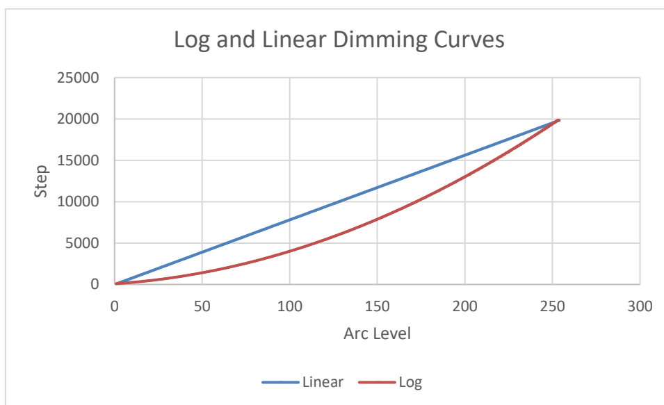
Figure 1. Log and Linear Dimming Curves
